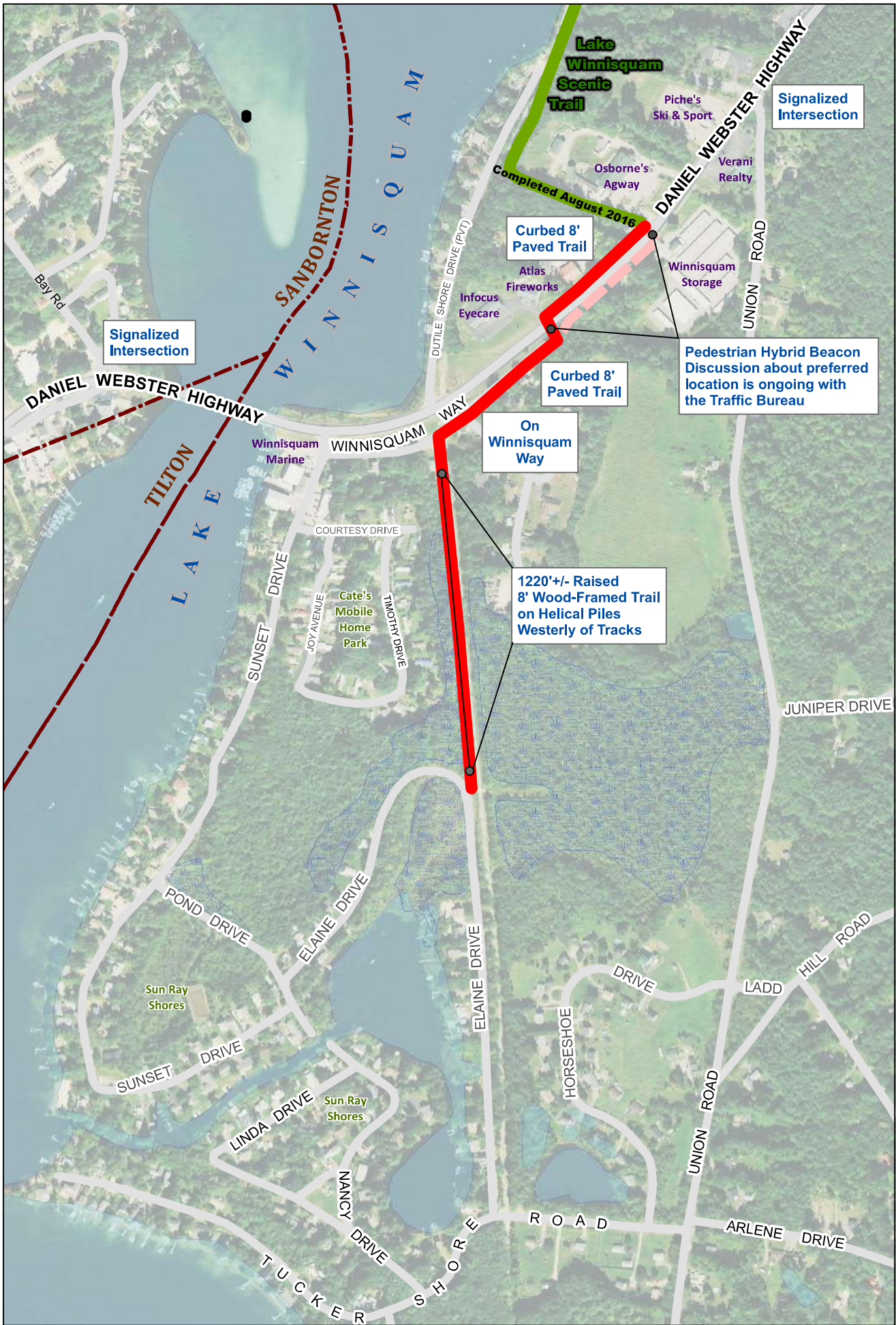
LAKE WINNISQUAM SCENIC TRAIL - PHASE 2 BELMONT, NEW HAMPSHIRE MARCH 2021
